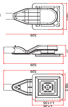
WR135SS Stainless Steel 135 x 135mm £149.00
