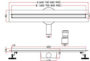
SLD60GB Slim linear drain - Gun Black 600x30mm £325.00
